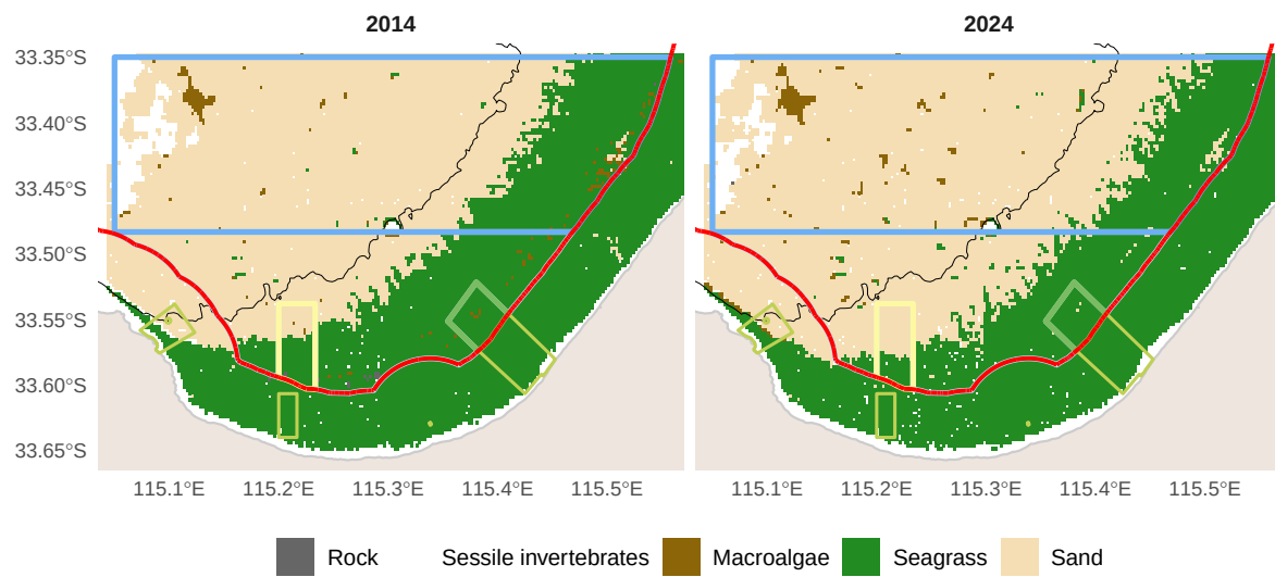
Figure 1: Predicted dominant habitat type
