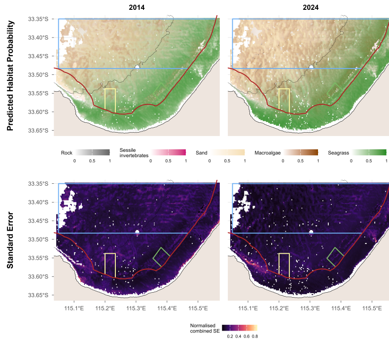
Figure 2: Predicted habitat distribution probability and uncertainty
